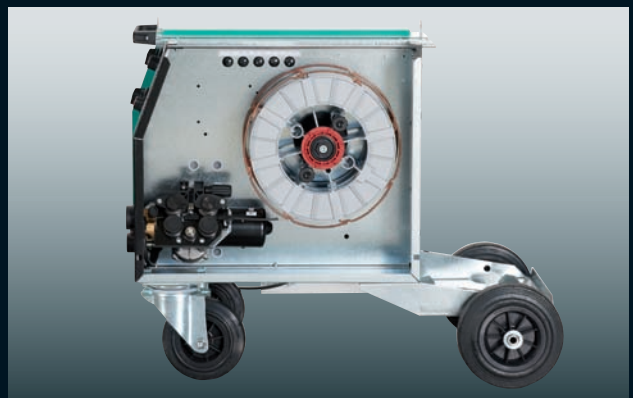
The wire feed system and wire spool mounting points are both open and easy to access.
