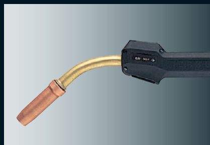
SB 307 G mixed gas: 280 A 60% duty cycle CO 2 : 300 A 60% duty cycle
